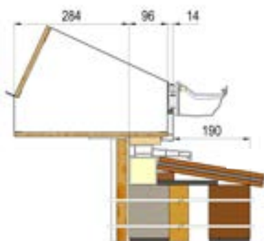
-190mm soffit
